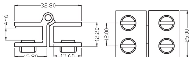
C3010B-06S-GG-180
