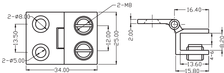
C3010B-06S-GW-90
