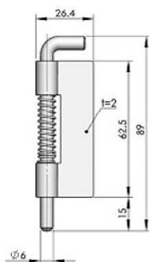
CL225-1-Y • Weld on • Left
