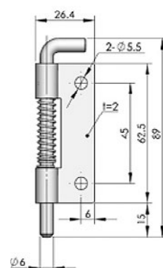
CL225-1A-Z • Mounting holes • Right
